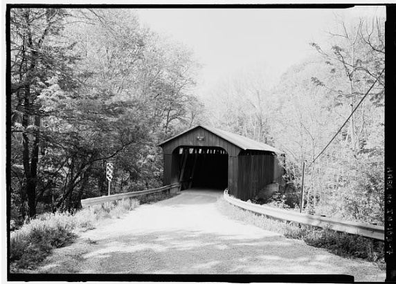
Pine Bluff Bridge (1886) Bainbridge vicinity, Putnam County, Indiana Joseph A. Britton, Builder Howe truss
