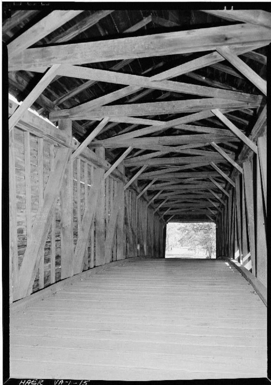
HUMPBAC BRIDGE. General interior view from east portal. Photograph by Jack Boucher, 1971
