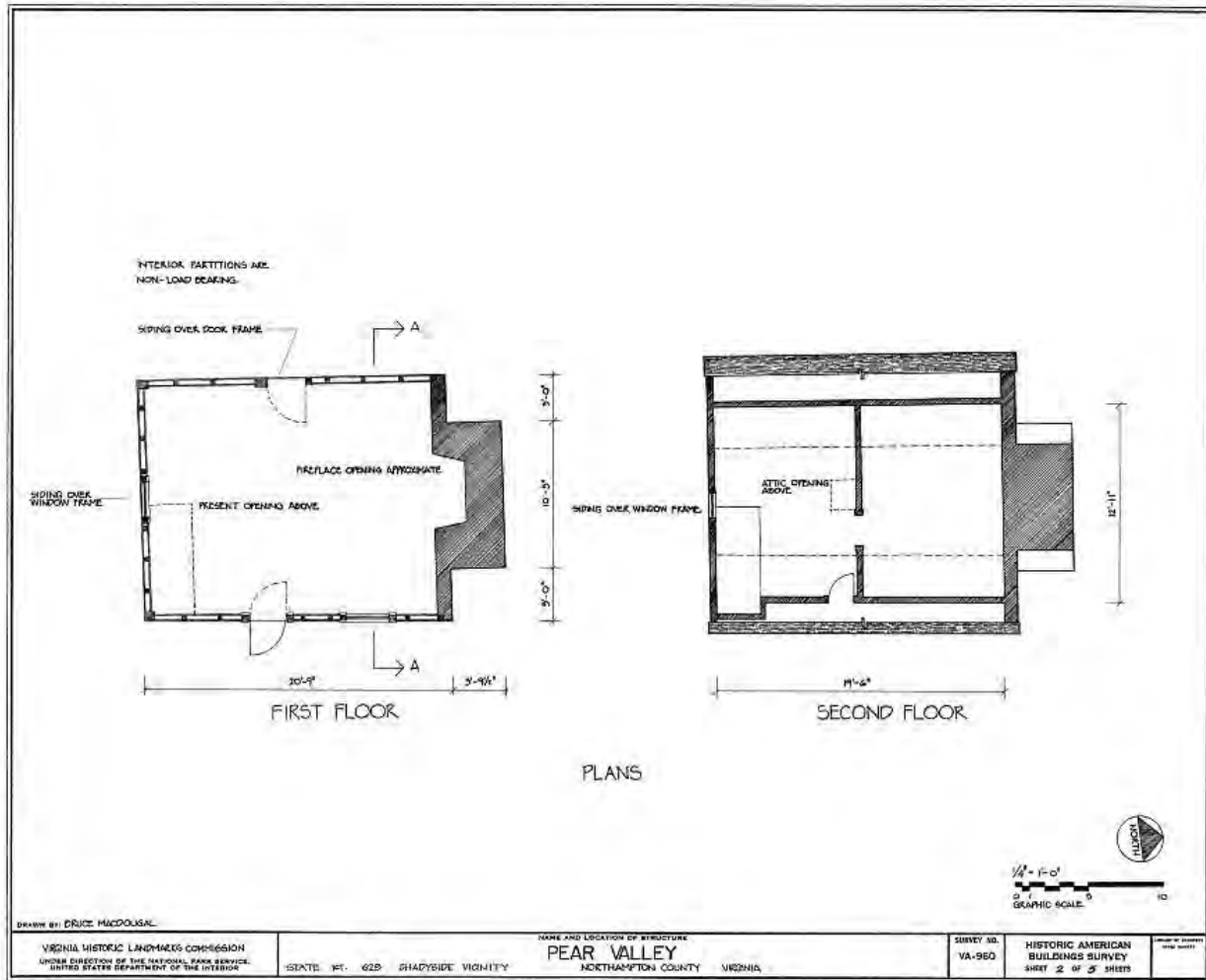
Pear Valley, floor plans, 1971 Historic American Buildings Survey (Bruce MacDougal, delineator)
