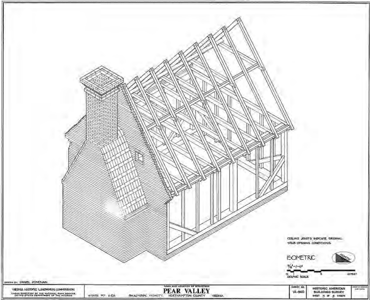
Pear Valley isometric, 1971 Historic American Buildings Survey (Daniel Donovan, delineator)
