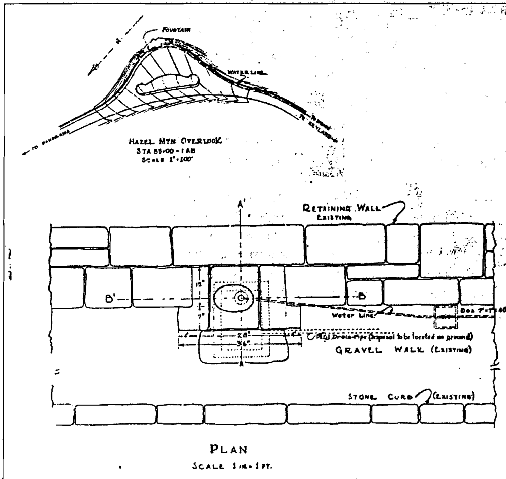
Fig. 6. Hazel Mountain Parking Overlook, with detailed plan of wall and water fountain (National Park Service, Technical Information Center, Denver).
