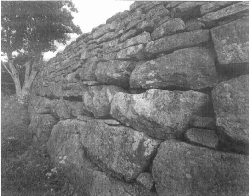
Retaining wall at Jewell Hollow. Photograph by William A. Faust II, 1996.
