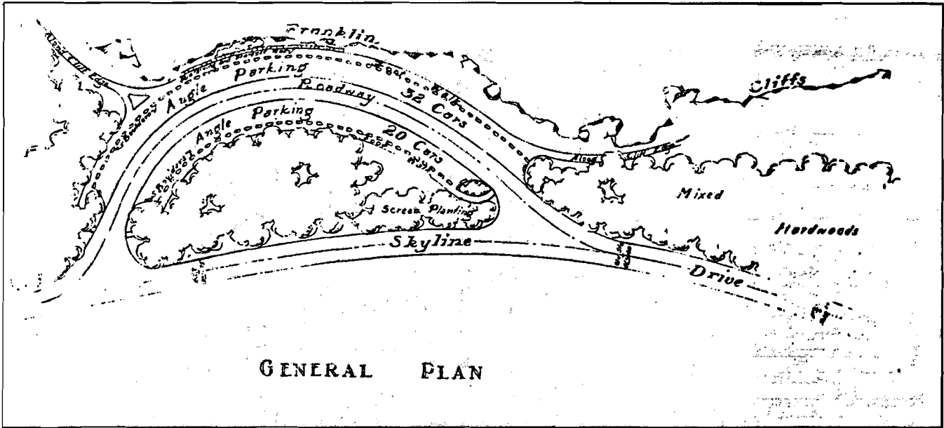
Fig. 5. Plan, Franklin Cliffs Parking Overlook, drawn by Roland W. Rogers, August 1934 (National Park Service, Technical Information Center, Denver).
