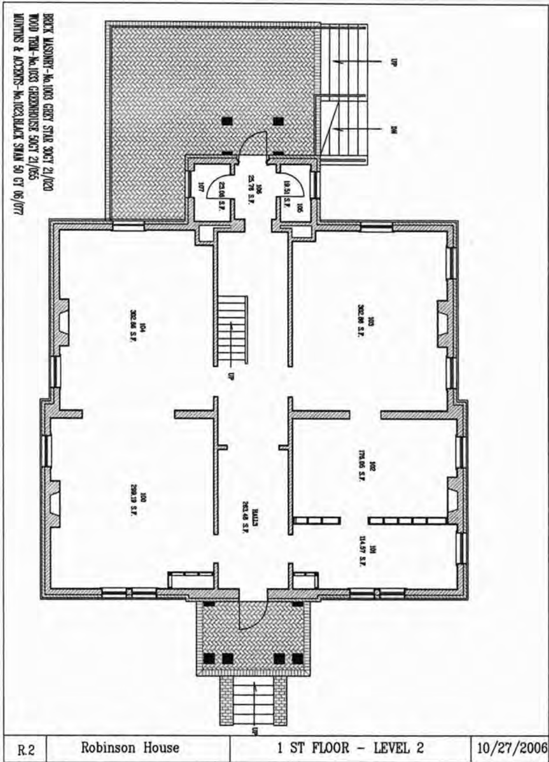
Fig. 2. Floor plan, first floor. Margaret R. and Robert M. Freeman Library VMFA.
