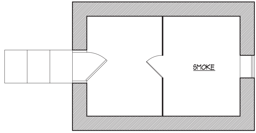
C3 JAMES SPRINGHOUSE FIRST FLOOR PLAN A201 1/4" = 1'-0"
