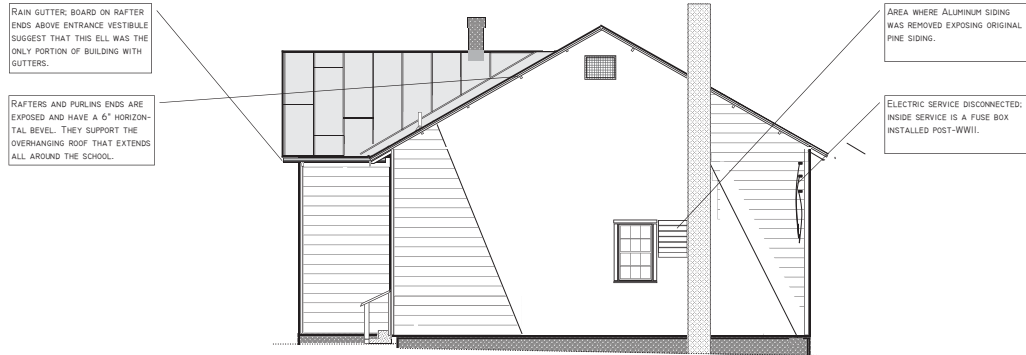
EAST ELEVATION
