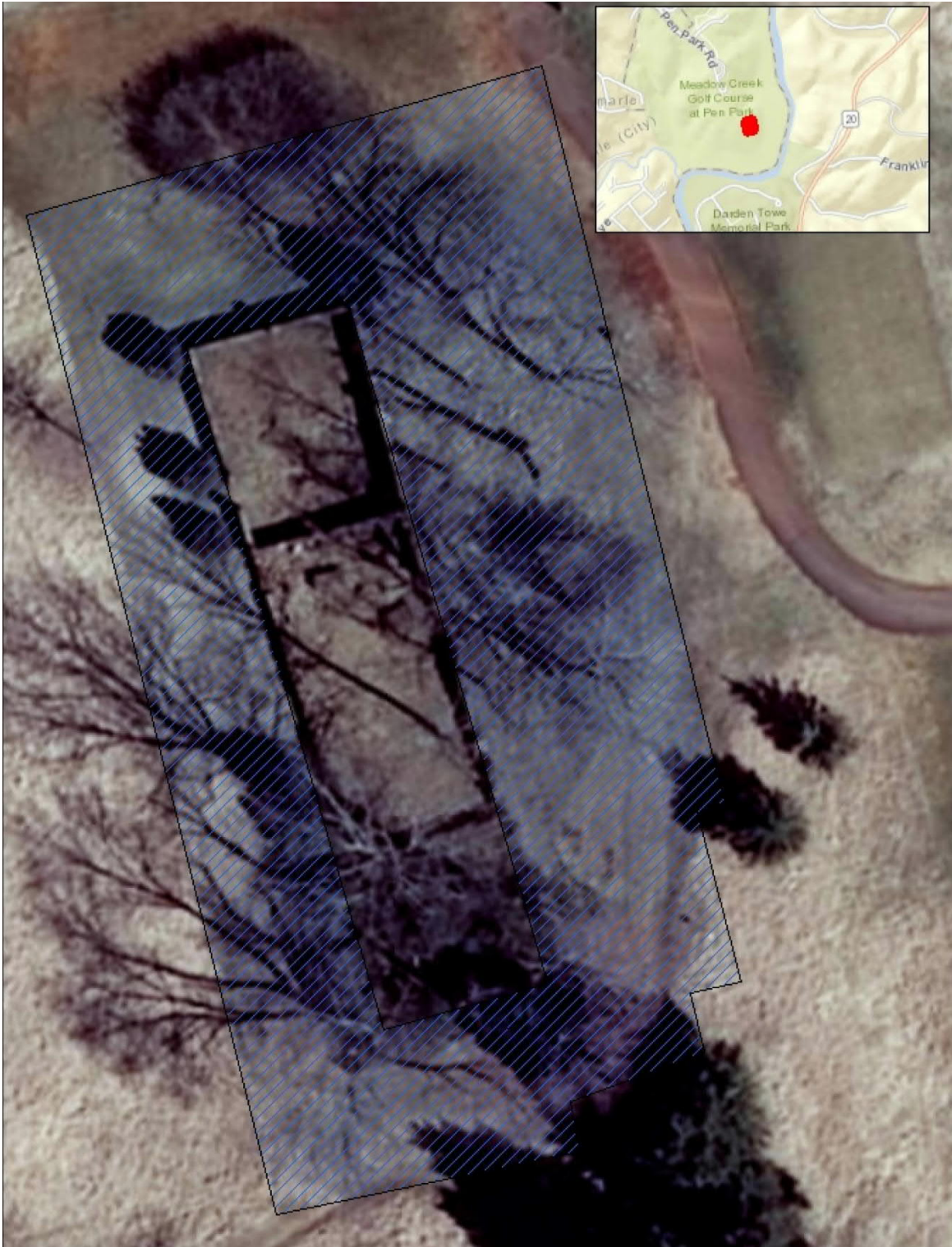
Figure #12: GPR Survey area (blue shading) surrounding the Pen Park cemetery.
